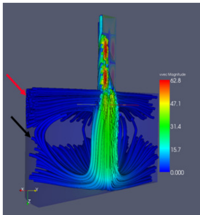
Figure 61. Secondary and Tertiary Flow Patterns—Jet Cross Section View. (The Red and Black Arrows Indicate the Secondary and Tertiary Flow Patterns, Respectively.)
