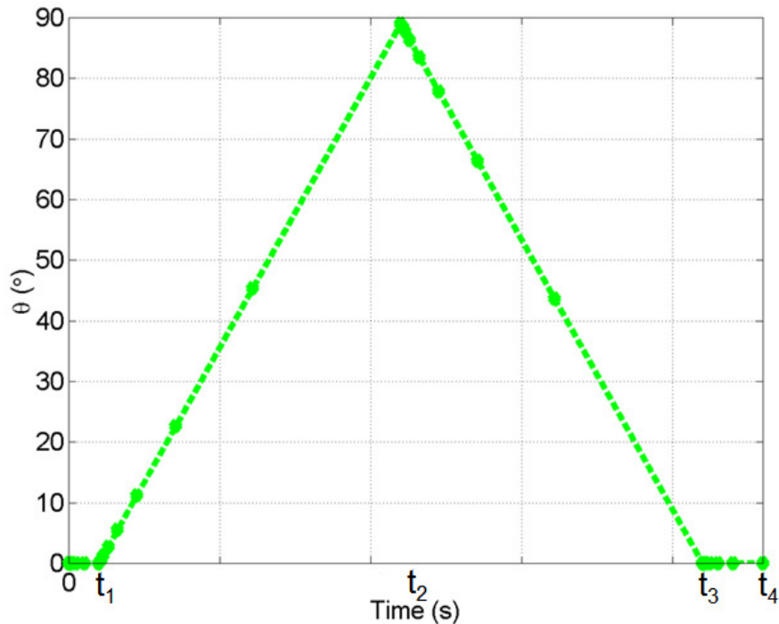
Figure 97. Dynamic Swirl Angle.
