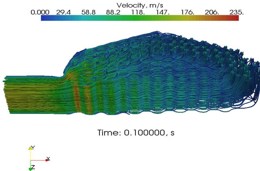
Figure 126. LP Net Velocity Streamlines.
