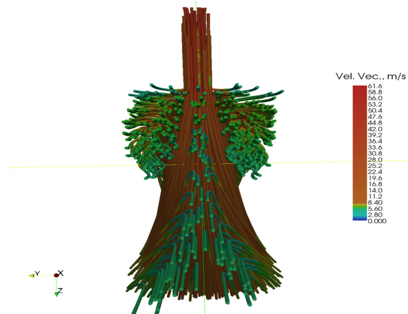
Figure 109. Crossflow Flowing around the Jet, Back View.
