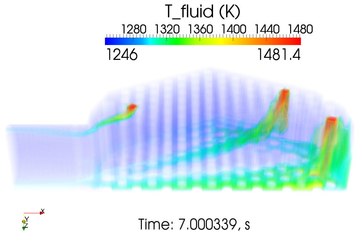
Figure 155. Volume Rendering of Fluid Temperature for the Three Hot Channels.
