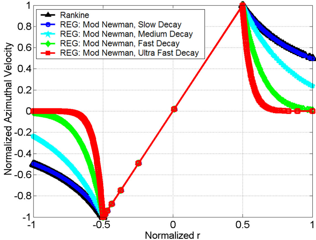
Figure 96. Modified Newman Vortex with Various Degrees of Decay.
